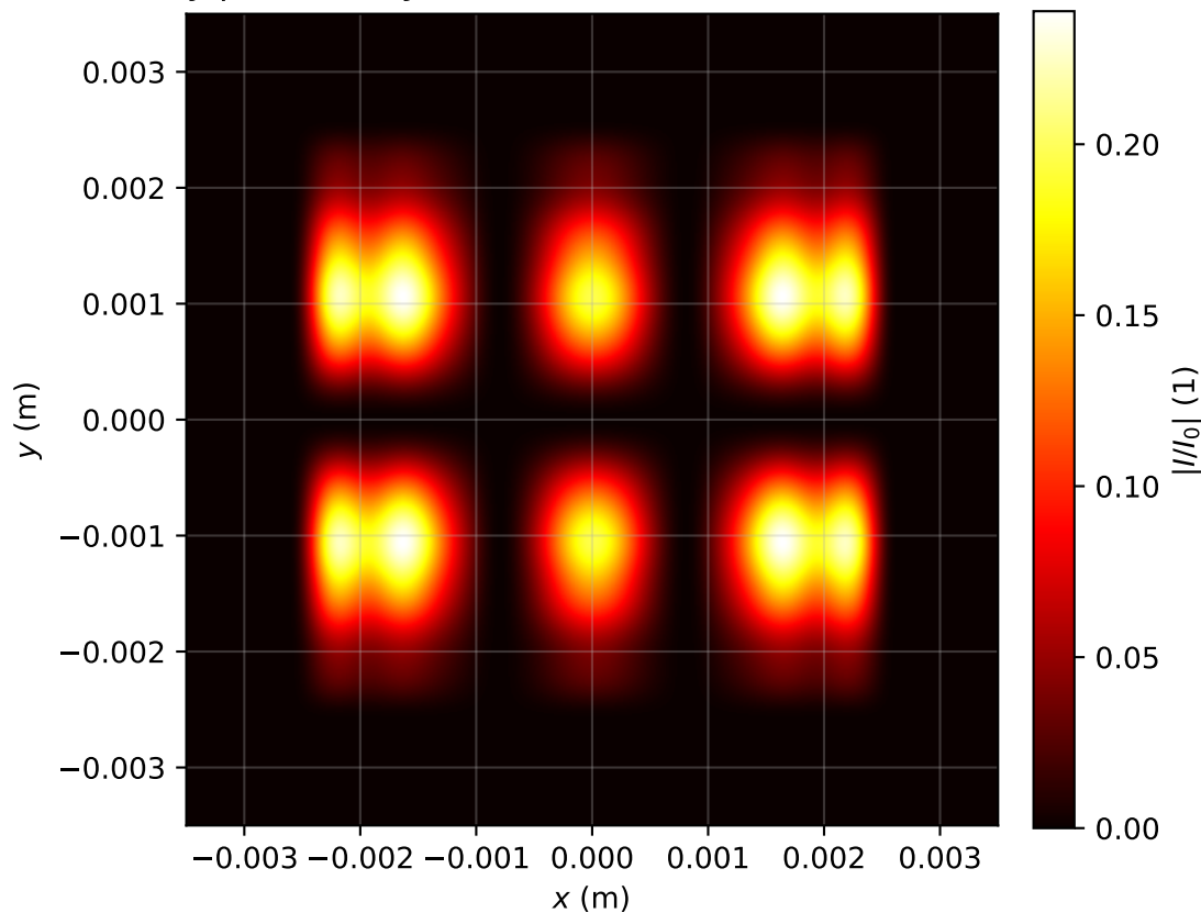
Intensity profile I(x, y, z = 3.981)/I_0 , P_{in}=1.0P_{cr} , artificial time
